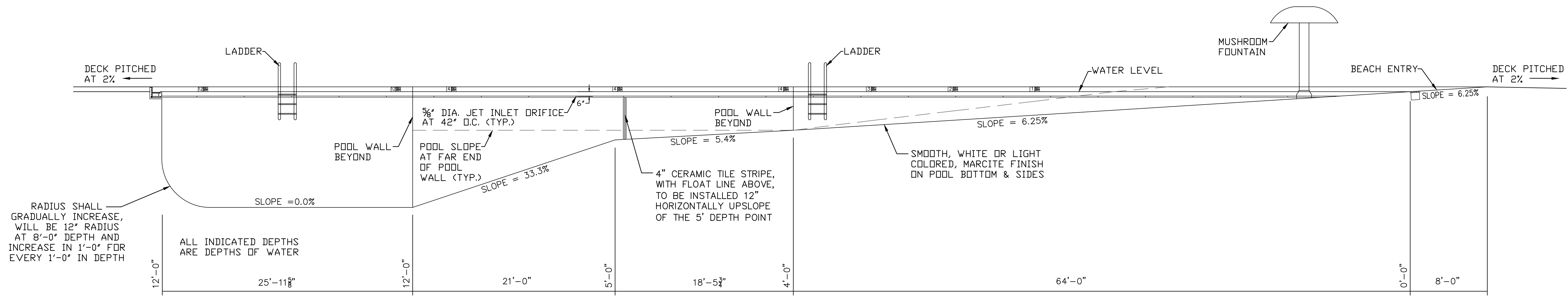
POOL SECTION VIEW A-A SCALE: 1"=6'
