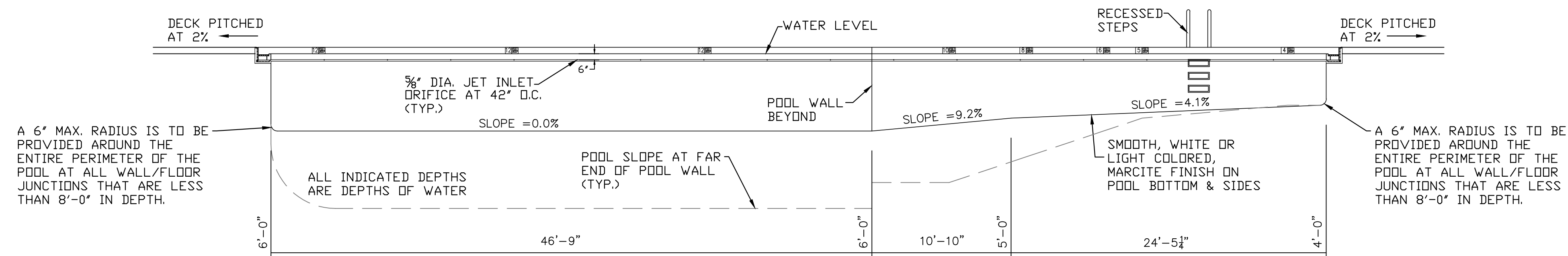
POOL SECTION VIEW A-A SCALE: 1"=6'
