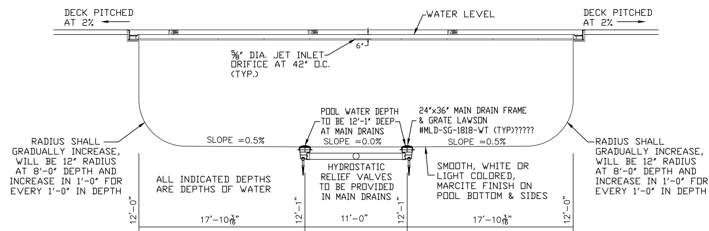
POOL SECTION VIEW D-D SCALE: 1"=6'
