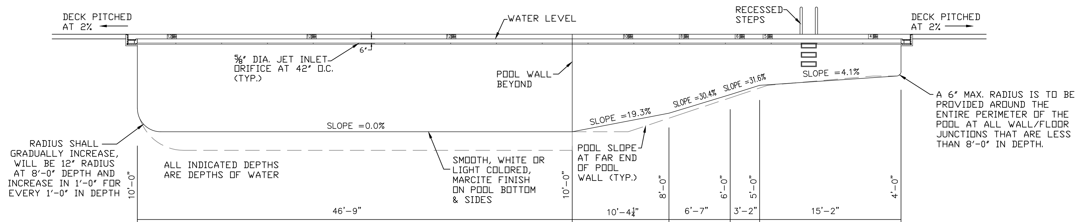
POOL SECTION VIEW C-C SCALE: 1"=6'
